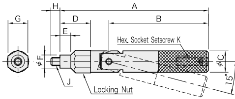
QLTL (Screw-In Handles)
