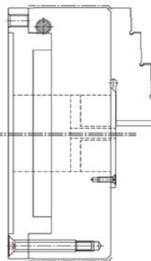
ZS Hi-Tru, with special seal for grinding machines, DIN 6350, cylindrical centre mount, form A
