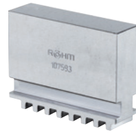
A09 Unstepped jaw BL, DIN 6350, unstepped, soft, material 16MnCr5
