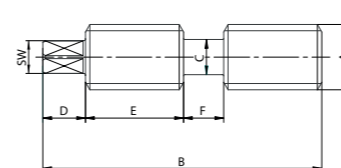
Adjusting spindle
