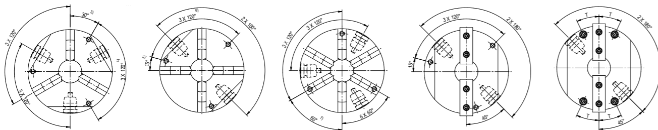
Position of the fastening screws for lathe chucks with cylindrical centring mount size 74-630
