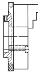
Dimensions KRF, cylindrical centre mount
