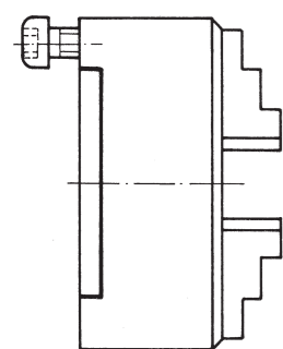
A09 DIN 6350, cylindrical centre mount, form A
