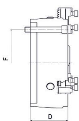
A08 Cylindrical centre mount
