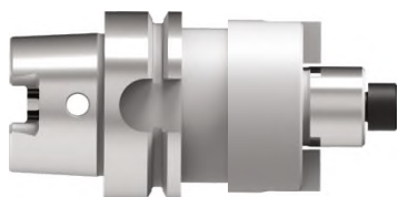
HSK-A100 DIN69893A
