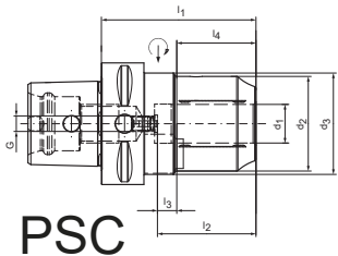
Ø 6+8+10+12+16 mm
