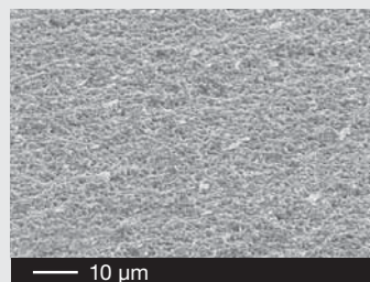
Detailansicht Feinstkornhartmetall (links) und Schichtaufbau TERAspeed (rechts). Detail of micor-grade carbide grade (left) and coating structure of TERAspeed (right).
