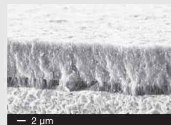
Detailansicht Feinstkornhartmetall (links) und Schichtaufbau TERAspeed (rechts). Detail of micor-grade carbide grade (left) and coating structure of TERAspeed (right).
